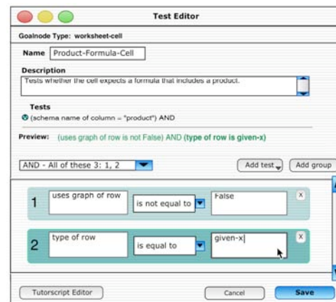
Figure 4. Rule Editor.
